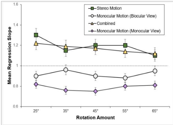
Mean Regression Slopes in Experiment
